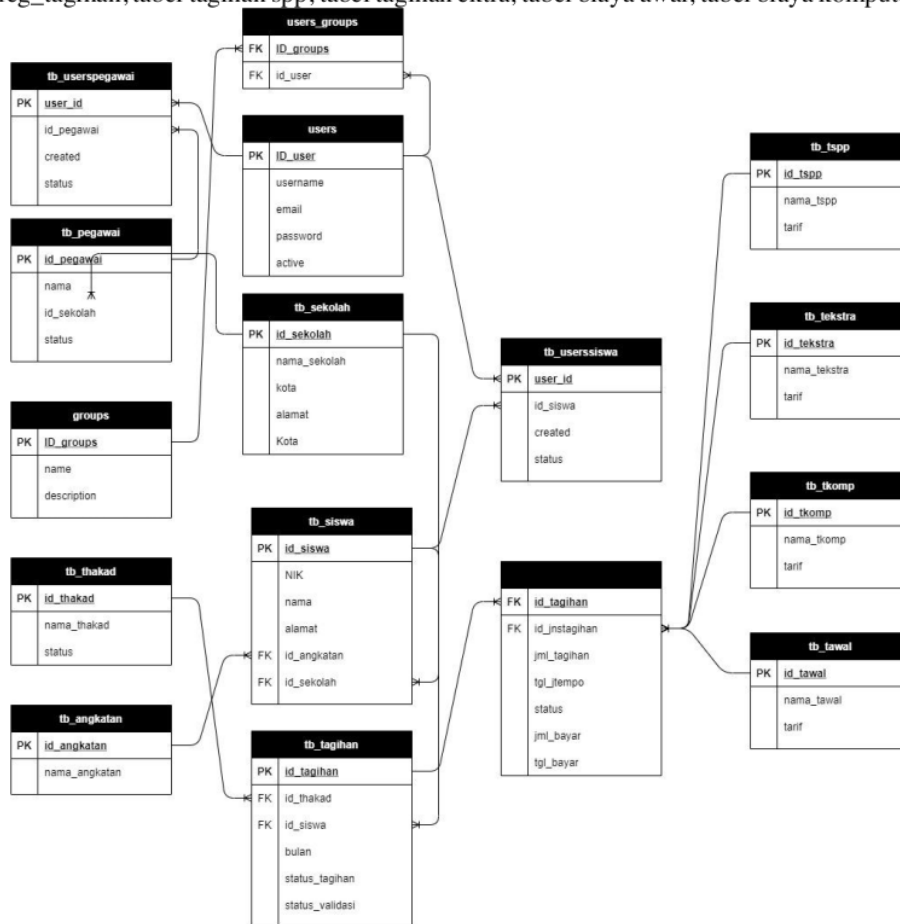
1 Gambar 7. ERD Physical sistem
