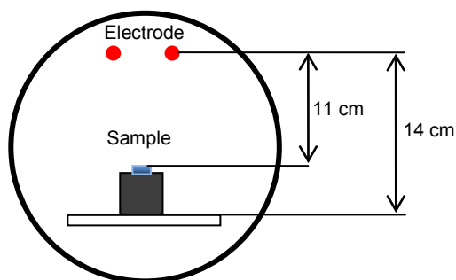
Fig. 1: Experimental set-up for plasma ashing/etching.
