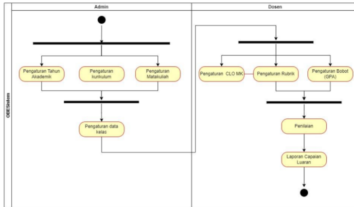
Gambar 3. Activity Diagram sistem (alur assessment , evaluasi)
