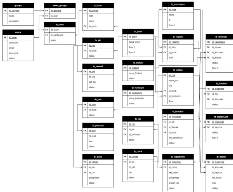
Gambar 4. Diagram ERD sistem
