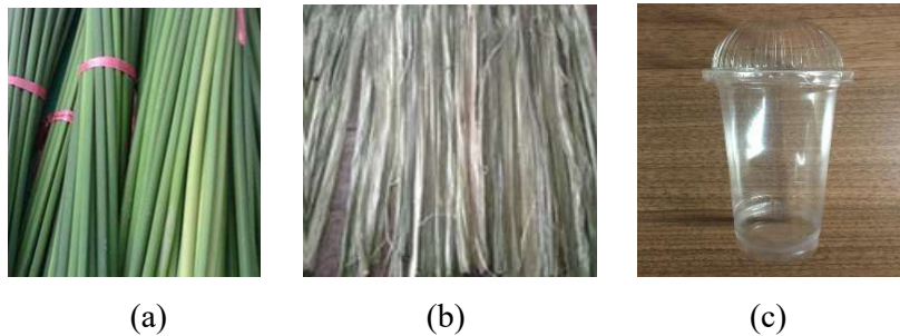
Gambar 4.1 Bahan komposit (a) Batang tanaman rumput payung (b) Serat batang tanaman rumput payung (c) Polypropylene (PP)
