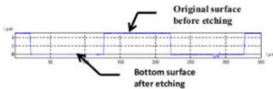
Fig. 12: Depth profile of micro-grooving pattern, plasma-etched onto the DLC coating when using the Cr-grooving pattern with W_G = 100\ \mu\text{m} and P_G = 200\ \mu\text{m} .
