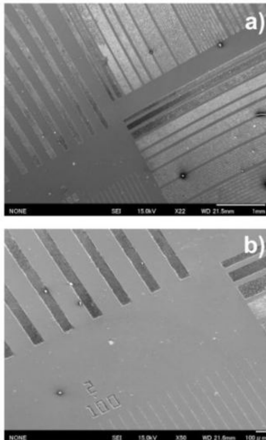
Fig. 11: SEM image of micro-patterns onto the DLC coatings by the oxygen plasma etching.
