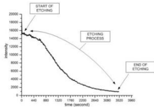
Fig. 16: Variation of detected CO-peak at 256.83 nm with duration time in etching process.
