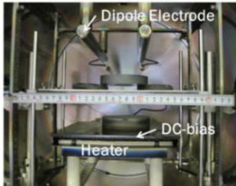
Fig. 2: Experimental set-up in this plasma etching system.
