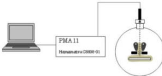
Fig. 3: Illustration of plasma diagnosis instrumentation attached to the present plasma etching system.
