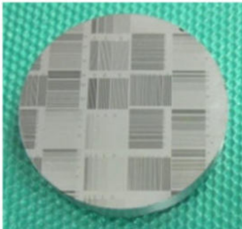
Fig. 5 Chromium masked SKD-11 specimen with variety of micro-groove pattern in the masking.
