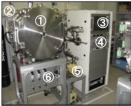
Fig.1: High density plasma etching system. 1: Chamber, 2: RF-plasma generator, 3: Control-panel, 4: Electric sources, 5: Evacuation system, 6: Gas supply.
