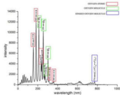
Fig. 6: Oxygen molecule governing state of plasmas.
