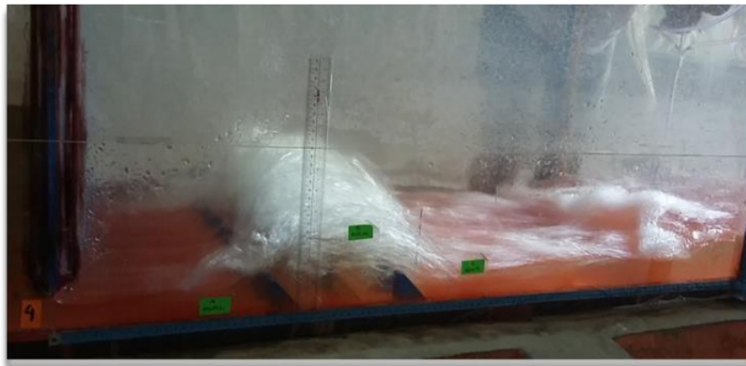
Figure 1. Trapezoid baffle block configuration in front of sluice gate
