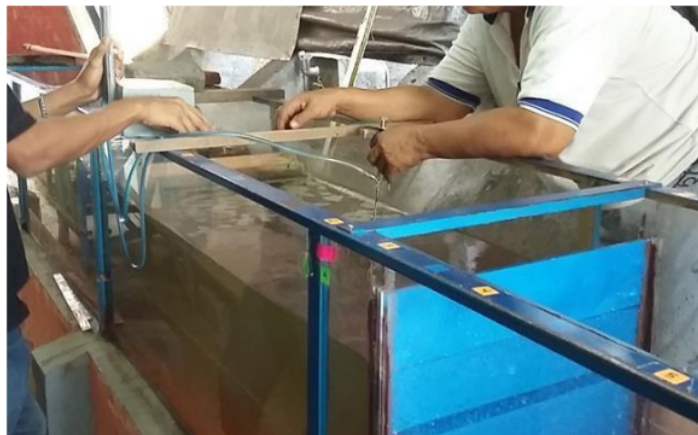
Figure 2. Water depth and velocity measurement for 12 section
